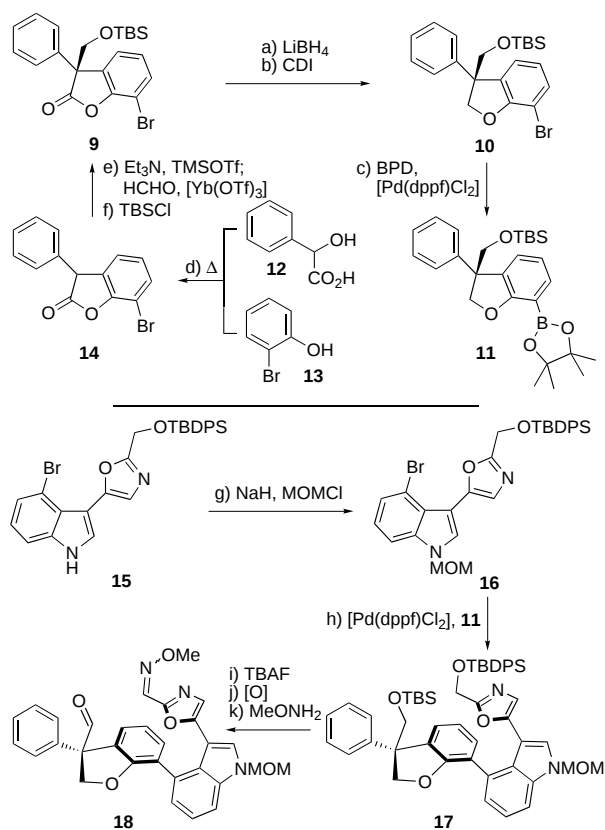
Scheme 3. Synthesis of key intermediate 18 : a) \text{LiBH}_4 (8.0 equiv), THF, 25^\circ\text{C} , 4 h, 95%; b) \text{CDI} (2.0 equiv), THF, reflux, 2 h, 95%; c) \text{BPD} (1.2 equiv), [\text{Pd}(\text{dppf})\text{Cl}_2] \cdot \text{CH}_2\text{Cl}_2 (0.2 equiv), \text{KOAc} (3.0 equiv), \text{DMSO} , 90^\circ\text{C} , 6 h, 70%; d) 12 (1.0 equiv), 13 (1.0 equiv), \text{H}_2\text{SO}_4 (70% aq.), 45 min, 42% (95% based on recovered 13 ); e) \text{Et}_3\text{N} (3.0 equiv), \text{TMSOTf} (1.2 equiv), \text{CH}_2\text{Cl}_2 , 0^\circ\text{C} , 1 h; then \text{HCHO} (37% in \text{H}_2\text{O} , 5.0 equiv), [\text{Yb}(\text{OTf})_3] (0.1 equiv), THF, 25^\circ\text{C} , 24 h, 78%; f) \text{TBSCl} (3.0 equiv), imidazole (6.0 equiv), DMF, 25^\circ\text{C} , 6 h, 95%; g) \text{NaH} (2.0 equiv), THF, 0^\circ\text{C} , 5 min; then \text{MOMCl} (2.0 equiv), THF, 0^\circ\text{C} , 10 min, 94%; h) 11 (1.0 equiv), [\text{Pd}(\text{dppf})\text{Cl}_2] \cdot \text{CH}_2\text{Cl}_2 (0.2 equiv), \text{K}_2\text{CO}_3 (5.0 equiv), DME, 110^\circ\text{C} , 8 h, 66%; i) \text{TBAF} (3.0 equiv), THF, 25^\circ\text{C} , 10 min, 93%; j) Dess–Martin periodinane (3.0 equiv), \text{NaHCO}_3 (10 equiv), \text{CH}_2\text{Cl}_2 , 25^\circ\text{C} , 1 h, 88%; k) \text{MeONH}_2 \cdot \text{HCl} (10 equiv), \text{DMSO} , 25^\circ\text{C} , 10 min, 91%. \text{CDI} = 1,1'-carbonyldiimidazole, \text{BPD} = bis(pinacolato)diboron, \text{dppf} = (diphenylphosphanyl)ferrocene, \text{LiHMDS} = lithium salt of 1,1,1,3,3,3-hexamethyldisilazane, \text{TBS} = tert -butyldimethylsilyl, \text{TBDPS} = tert -butyldiphenylsilyl, \text{MOM} = methoxymethyl, \text{TBAF} = tetrabutylammonium fluoride.
