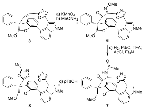
Scheme 2. Initial model studies which led to the complete heteroaromatic skeleton ( 8 ) of diazonamide A: a) \text{KMnO}_4 (6.0 equiv), \text{Ac}_2\text{O} , 0^\circ\text{C} , 2 h, 35%; b) \text{MeONH}_2 \cdot \text{HCl} (20 equiv), \text{EtOH} , 25^\circ\text{C} , 12 h, 95%; c) \text{Pd/C} (10%, 2.0 equiv), \text{H}_2 (3.0 atm), \text{TFA}/\text{MeOH} (1:20), 25^\circ\text{C} , 12 h; then \text{AcCl} (3.0 equiv), \text{Et}_3\text{N} (3.0 equiv), \text{CH}_2\text{Cl}_2 , 25^\circ\text{C} , 30 min, 80%; d) p\text{TsOH} , benzene, 80^\circ\text{C} , 20 h, 50%. \text{TFA} = trifluoroacetic acid, p\text{TsOH} = p -toluenesulfonic acid.
